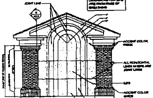
ENLARGED ELEVATION SCALE: 1/4" = 1'-0"
