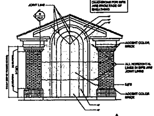
ENLARGED ELEVATION SCALE: 1/4" = 1'-0"
