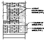
TYPICAL WINDOW BRICK QUIONS DETAIL SCALE: 1/4" = 1'-0"
