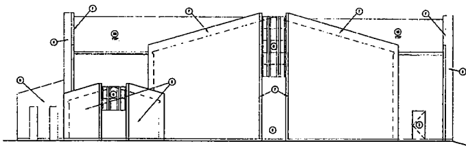
EXISTING NORTH ELEVATION SCALE: 1/8" = 1'-0"
