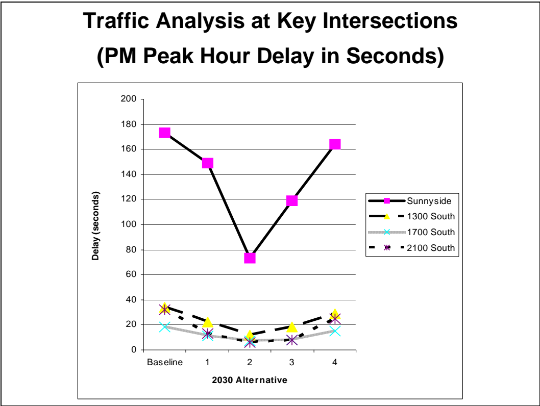
Figure 9 Intersection Delay
